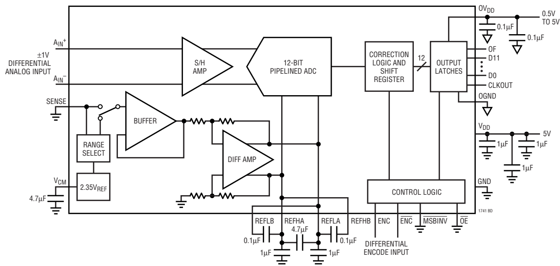
65Msps, 12-Bit ADC with a \pm 1\text{V} Differential Input Range
